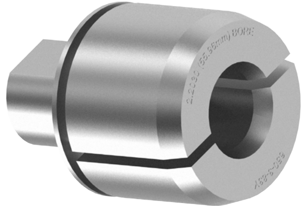
650-3-83Y Locator, Cam, Expanding (2.2030 - 2.2040" bore) (55.96 - 55.98mm)
